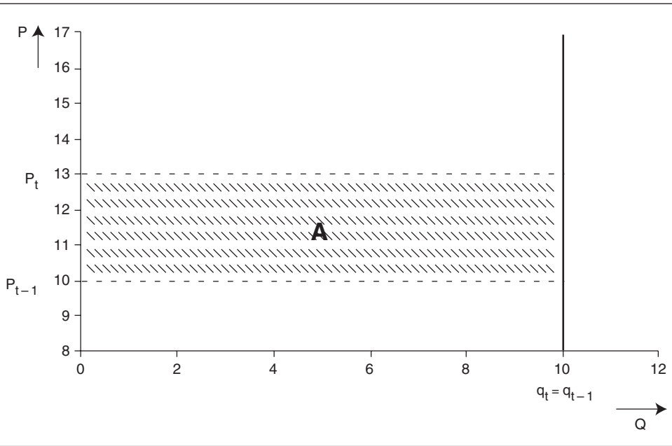
FIGURE 7-1 Paasche Variation in Consumption Expenditure
