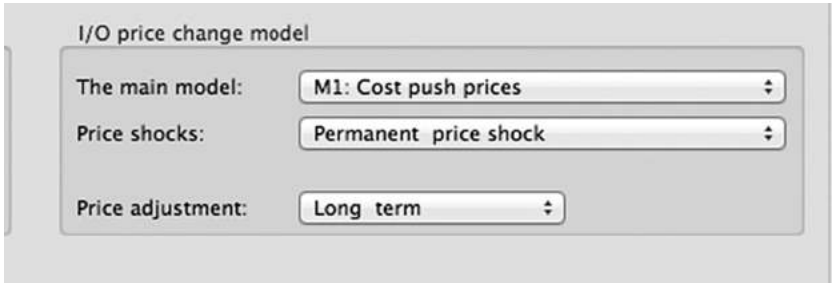
FIGURE 7-4 The SUBSIM “I/O Price Change Model Menu”
