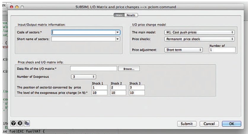
FIGURE 7-3 The SUBSIM “Price Shocks” Submenu in the “I/O Price Change Model”
